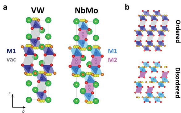
Fig. 6 (a) Average crystal structure of Ba_3VWO_{8.5} (VW) and Ba_3NbMoO_{8.5} (NbMo). The green spheres are the Ba atoms, while the oxygen atoms are represented by red (O1), orange (O2) and yellow (O3) spheres. Blue and light blue polyhedra represent the average M1O_x units created by partial occupation of O2 and O3. The grey polyhedra in VW represents the empty octahedral cavities. M2O_6 octahedra are represented in magenta in NbMo. (b) Representation of the ordered stacking of palmierite-like layers and cation vacancies in Ba_3VWO_{8.5} (top), and of a possible disordered arrangement of face-sharing and isolated polyhedral units in Ba_3NbMoO_{8.5} (bottom). O3 is represented at 6c for simplicity.
