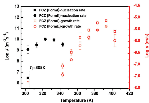
Fig. 4 Nucleation rate and crystal growth rate for amorphous FCZ as a function of temperature (black circles represent the nucleation rates of Form II, black squares represent the estimated upper bound of the nucleation rate of Form I, red empty circles represent the crystal growth rates of Form II, and red empty squares represent the crystal growth rates of Form I) ( n = 3 ).
