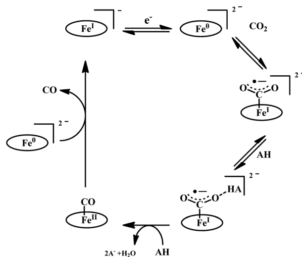
Scheme 7 Proposed mechanistic pathway for the reduction of \text{CO}_2 to CO by Fe-porphyrin electrocatalysts.
