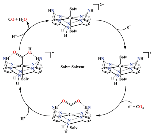
Scheme 13 Proposed mechanistic pathway for electrocatalytic \text{CO}_2 reduction to CO by azacalix-pyridine based macrocycles.
