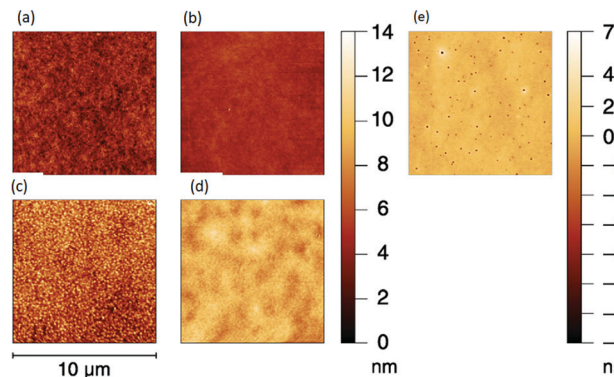
Fig. 15 AFM images of (a) PEDOT:PSS (b) SimCP2:FlrCP2 (c) TPBi from MeOH (d) TPBi from MeOH-AA and (e) TPBi from 1-Prop-FA (reprinted with permission from the ref. 43).
