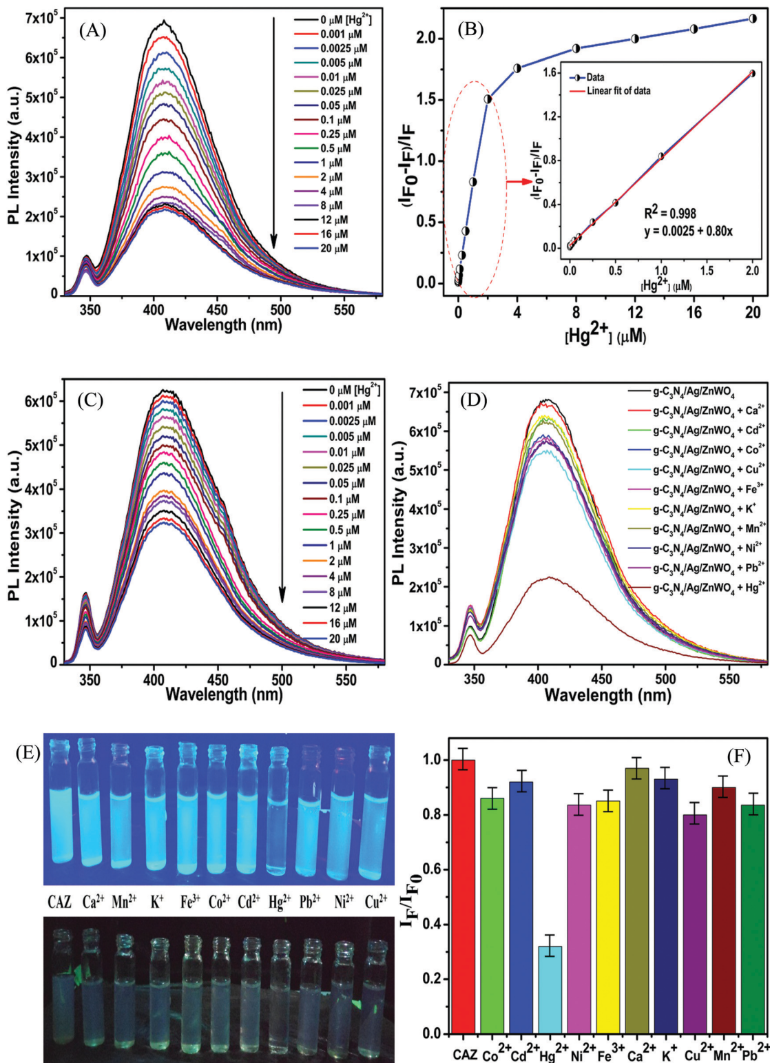
Fig. 7 (A) and (C) PL intensity responses of \text{g-C}_3\text{N}_4/\text{Ag/ZnWO}_4 in phosphate buffer (pH = 7.2) and tap water, respectively on the addition of different amounts of \text{Hg}^{2+} , \lambda_{\text{ex}} = 310 \text{ nm} , (B) calibration curve of \text{g-C}_3\text{N}_4/\text{Ag/ZnWO}_4 for the detection of \text{Hg}^{2+} (inset is a linear plot of relative intensity vs. conc. of \text{Hg}^{2+} ), (D) PL emission of \text{g-C}_3\text{N}_4/\text{Ag/ZnWO}_4 in the presence of different metal ions individually ( \lambda_{\text{ex}} = 310 \text{ nm} , [\text{M}^{n+}] = 10 \mu\text{M} ), (E) photographic image of \text{g-C}_3\text{N}_4/\text{Ag/ZnWO}_4 in phosphate buffer under 365 nm light (upper panel) and white light in the presence of different metal ions (10 \mu\text{M} ) (lower panel), and (F) bar diagram of the relative PL emission intensities (I_F/I_0) of \text{g-C}_3\text{N}_4/\text{Ag/ZnWO}_4 in the presence of various metal ions (10 \mu\text{M} ).
