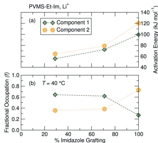
Fig. 8 (a) Activation energies and (b) fractional occupation at 40 °C of the two \text{Li}^+ components as a function of imidazole grafting density, extracted from ^7\text{Li} T_{1\rho} measurements as a function of temperature. Lower grafting density results in higher mobility and occupation of the more mobile Li environment. All samples consist of a 0.1 Li: monomer ratio of LiTFSI added to the polymer.
