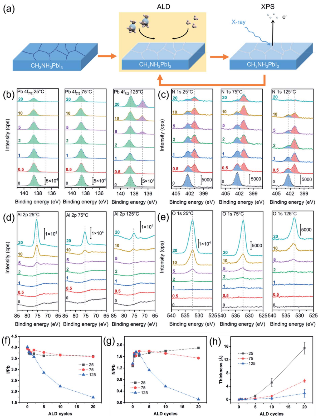
Fig. 1 (a) Schematic of the in situ experimental procedure. High-resolution XPS core-level spectra of (b) \text{Pb } 4f_{7/2} , (c) \text{N } 1s , (d) \text{Al } 2p , and (e) \text{O } 1s taken from 0 cycles ( i.e. , initial surface) through 20 cycles of ALD of \text{Al}_2\text{O}_3 on \text{MAPbI}_3 . The deposition temperatures were 25 °C, 75 °C and 125 °C. Atomic ratios of (f) \text{I/Pb} and (g) \text{N/Pb} and (h) the equivalent thickness of the deposited \text{Al}_2\text{O}_3 with respect to the number of the ALD cycles.
