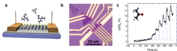
Fig. 4 (a) Schematic illustration and (b) optical image of the \text{MoS}_2 monolayer device. (c) Response of gas sensors to the exposure of acetone. Conductivity change of the \text{MoS}_2 sensor upon exposure to a sequence of pulses of acetone concentration from 0.02% P_0 (50 ppm) to 2% P_0 (5000 ppm, black line). Dashed blue line: pulse interval (20 s on/40 s off) and the corresponding concentrations. 52 Adapted with permission from ref. 52. Copyright 2013 American Chemical Society.
