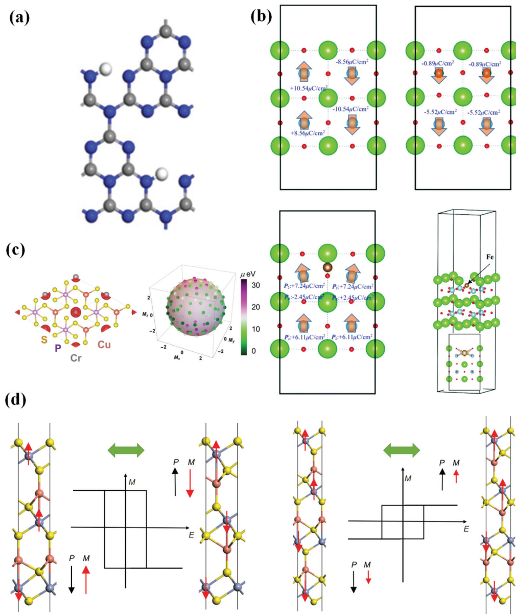
Fig. 2 Several 2D ferromagnetic–ferroelectric multiferroic materials in recent years. (a) Optimized structure of C 6 N 8 H. Reproduced with permission. 33 2017, American Chemical Society. (b) Ferroelectric characteristics of 2D BaTiO 3 ultrathin film without and with Fe. Reproduced with permission. 34 Copyright 2020, The Royal Society of Chemistry. (c) Ferroelectric and magnetic characteristics of monolayer CuCrP 2 S 6 . Reproduced with permission. 35 Copyright 2018, AIP Publishing. (d) Geometric structures and multiferroic conversion of Cu 2 (CrS 2 ) 3 (left) and Cu 3 (CrS 2 ) 4 (right) thin films. Reproduced with permission. 36 Copyright 2020, China Science Publishing & Media.
