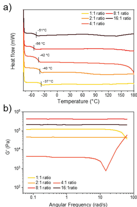
Fig. 3 Thermal and rheological properties of C_6E-3T networks. (a) DSC thermograms of the 2nd heating cycle from -80 to 180 °C, 10\ ^\circ C\ min^{-1} . (b) Frequency sweep analysis of films showing storage modulus versus frequency at 25 °C (1% strain from 0.1 to 10 Hz, or 0.06 to 62 rad\ s^{-1} ).
