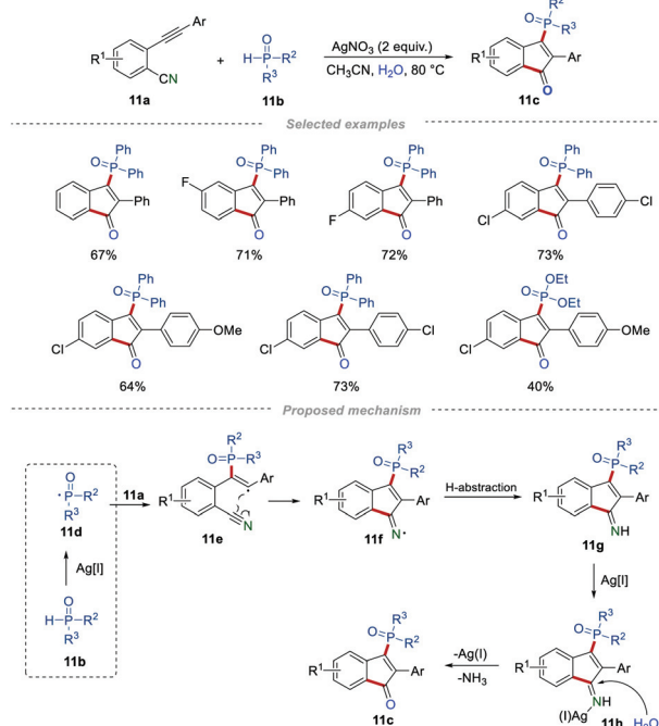
Scheme 11 The synthesis of phosphinylated indenones.
