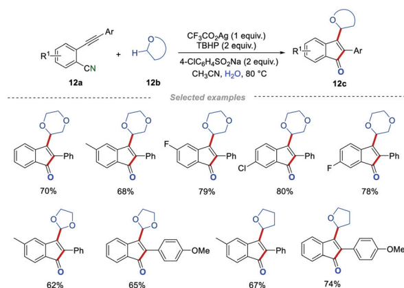
Scheme 12 The construction of 3-alkylated indenones.
