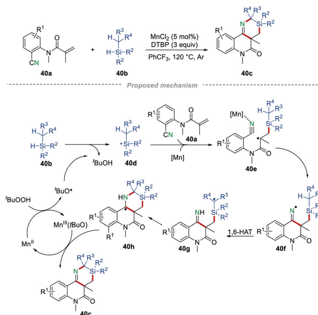
Scheme 40 The construction of silicon/nitrogen heterocycles.
