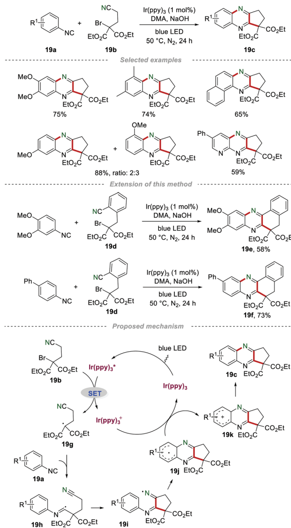
Scheme 19 The synthesis of fused quinoxaline derivatives.
