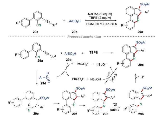
Scheme 29 The construction of 3-sulfonated cyclopenta[gh]phenanthridines.
