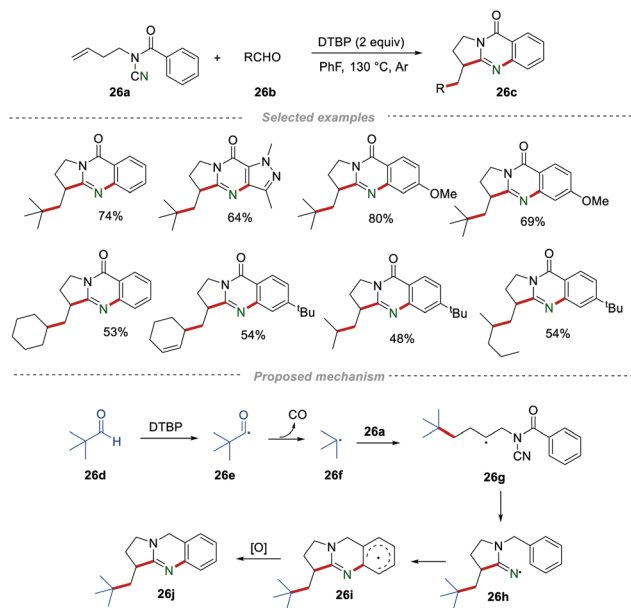
Scheme 26 The preparation of alkyl-substituted quinazolinones.
