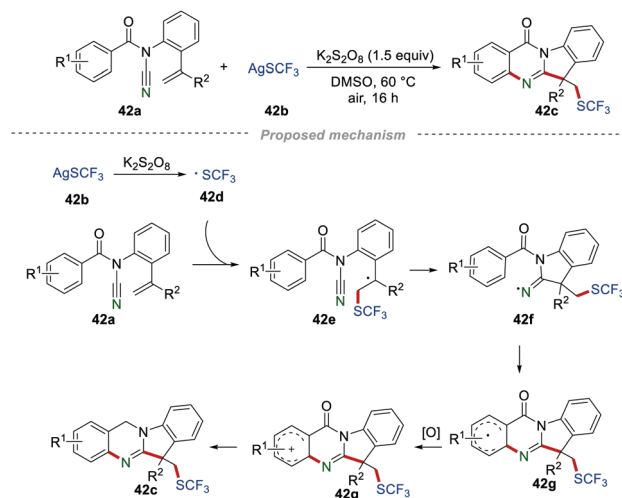
Scheme 42 Synthesis of SCF 3 -substituted tryptanthrin derivatives.
