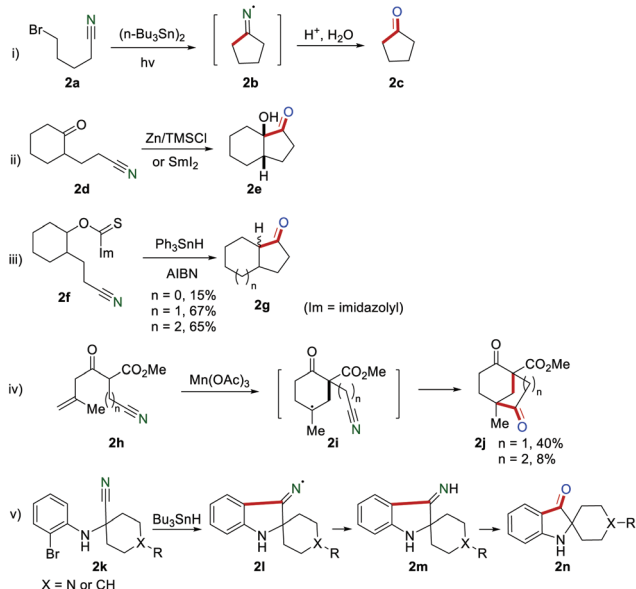
Scheme 2 Early studies on the iminyl radical for the construction of five-membered cyclic ketones.
