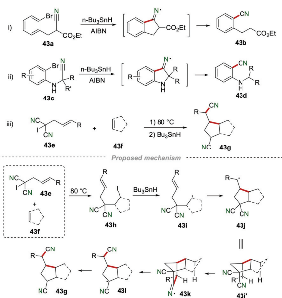
Scheme 43 Remote cyano migration to access nitriles.
