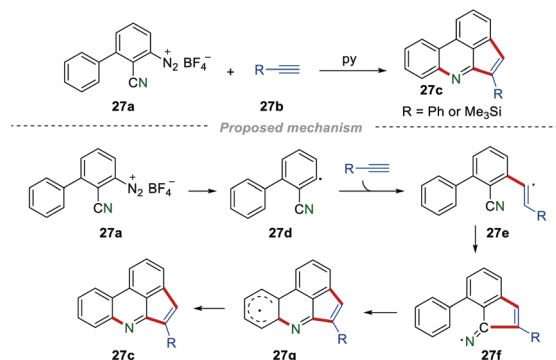
Scheme 27 The construction of cyclopentaphenanthridines.
