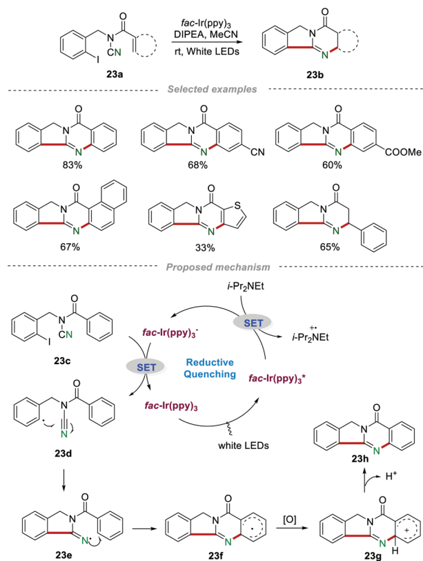
Scheme 23 The construction of quinazolinones via visible-light-promoted radical cyclization.
