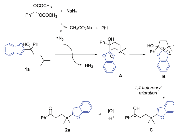
Scheme 5 Proposed mechanism.
