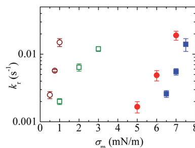
Fig. 11 The effects of the constant-mechanical-tension ( \sigma_m )-induced rupture of GUVs. The \sigma_m -dependent k_r values for 40%DLPG/60% DTPC-GUVs (○), 10%DLPG/90%DTPC-GUVs (□), 40%DOPG/60% DOPC-GUVs (●), and 10%DOPG/90%DOPC-GUVs (■). Mean k_r values with standard errors for each tension were determined using three independent experiments, each of which was conducted using 20 GUVs for each tension. This figure has been adapted from ref. 103 with permission from American Chemical Society, copyright 2016.
