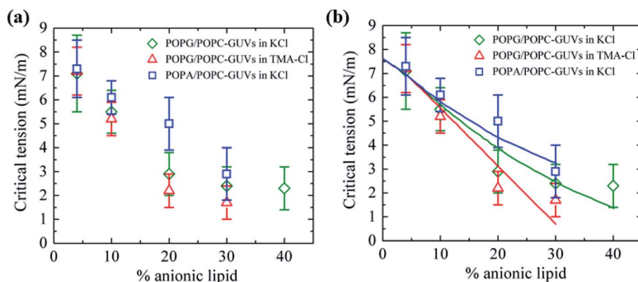
Fig. 17 The anionic-lipid-dependent critical tension for the rupture of GUVs using the micropipette technique. (a) POPG/POPC in KCl ( \circ ), POPG/POPC in TMA-Cl ( \Delta ), and POPA/POPC-GUVs in KCl ( \square ). (b) The experimental anionic-lipid-dependent critical tension data for POPG/POPC in KCl ( \circ ), POPG/POPC in TMA-Cl ( \Delta ), and POPA/POPC-GUVs in KCl ( \square ), fitted using eqn (14). The images in a and b have been adapted from ref. 119 with permission from The Biophysical Society (published by Elsevier Inc), copyright 2002.
