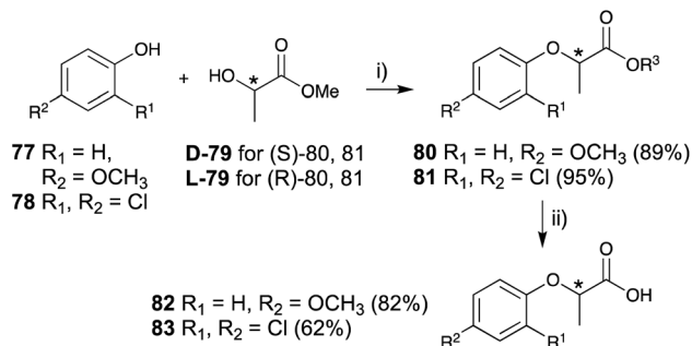
Fig. 12 Asymmetric synthesis of lactisole and (2-(2,4-dichlorophenoxy)propionic acid) derivative. (i) (1) \text{PPh}_3 , \text{CH}_2\text{Cl}_2 , 0^\circ\text{C} , 10 min, (2) DEAD, rt, 12 h, (ii) \text{K}_2\text{CO}_3 , \text{CH}_3\text{OH} , \text{H}_2\text{O} , reflux, 2 h.
