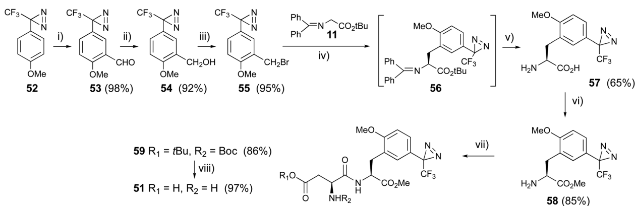
Fig. 8 Synthesis of trifluoromethyldiaziriny aspartame derivative. (i) Cl 2 CHOMe, TiCl 4 , 0 °C, 1 h, (ii) NaBH 4 , EtOH, rt, 4 h, (iii) CBr 4 , Ph 3 P, CH 2 Cl 2 , rt, 4 h, (iv) phosphazene base BTTPP, o -allyl- N -(9-anthracenylmethyl)chinchonidium bromide, CH 2 Cl 2 , –78 °C, 8 h, (v) TFA, 0 °C, 2 h, (vi) SOCl 2 , MeOH, rt, 8 h, (vii) N -Boc-L-Asp(OtBu)OSu, (i-Pr) 2 NEt, THF, rt, 8 h, (viii) TFA, 0 °C, 3 h.
