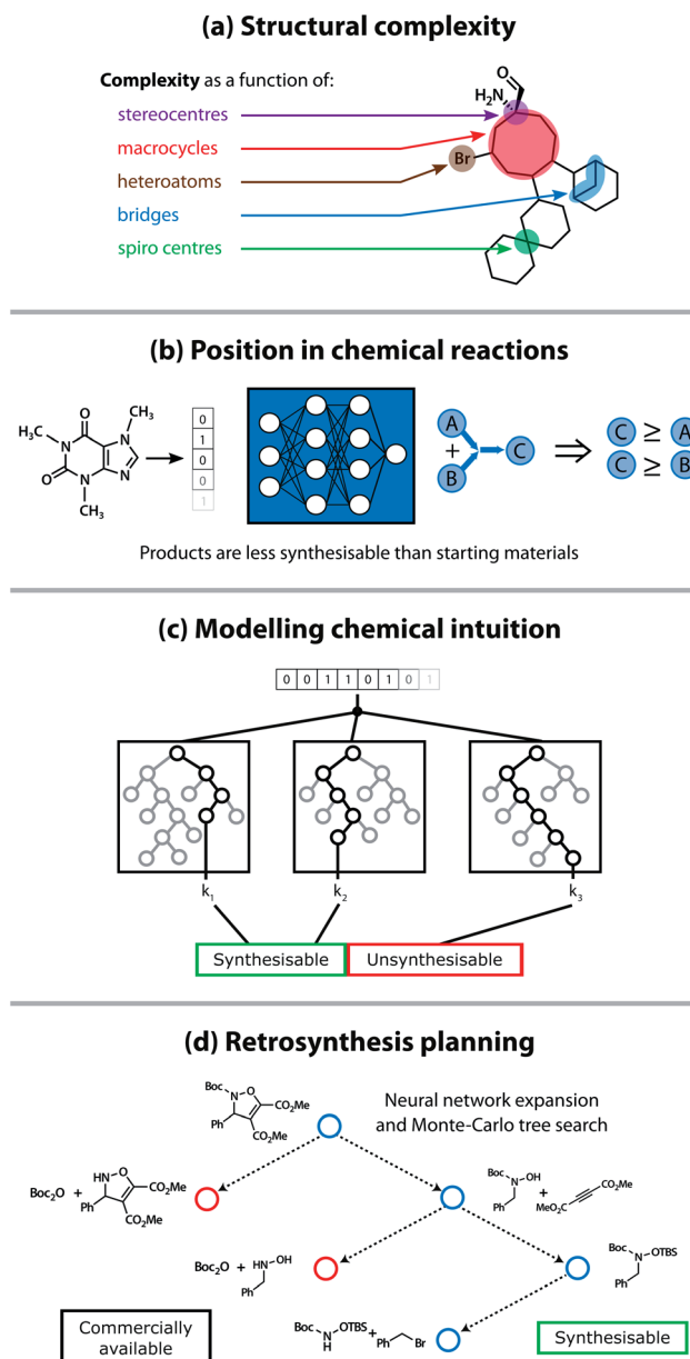
Fig. 2 Four approaches used to calculate the synthetic accessibility of organic compounds: (a) as function of the number of complex structural motifs present in the molecule; (b) deep neural networks trained on extensive reaction databases (reported and proprietary); (c) modelling the decision making process of expert chemists (the “chemical intuition”); (d) by identifying viable reaction pathways using automated retrosynthesis planning tools.
