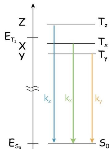
Scheme 1 Typical energy diagram for a triplet state (T 1 ), showing the lifting of the degeneracy of the sublevels in the case of an orthorhombic D-tensor. The ground state S 0 is also presented. E T1 – E S0 is in the order of 10 4 cm –1 , whereas |Z – X| is in the order of fractions of cm –1 . The scheme represents the case of the ZFS parameter D < 0.
