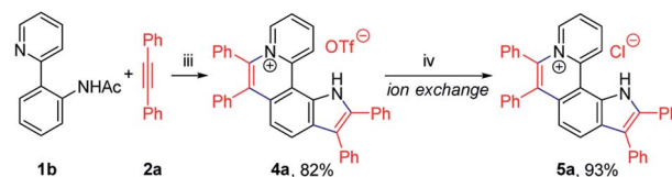
Scheme 2 Rh-Catalyzed cyclization of 2-(pyridin-2-yl)aniline ( 1 ) with 1,2-diphenylacetylene ( 2a ). Reaction conditions: (i) 1a (0.1 mmol), 2a (0.2 mmol), [Cp*RhCl 2 ] 2 (5 mol%), and AgOTf (0.12 mmol) in t -AmOH (1.5 mL) at 120 °C for 24 h under O 2 ; (ii) 1a (0.1 mmol), 2a (0.2 mmol), [Cp*RhCl 2 ] 2 (5 mol%), AgOTf (0.12 mmol), and Ac 2 O (0.5 mmol) in t -AmOH (1.5 mL) at 120 °C for 24 h under O 2 ; (iii) 1b (0.1 mmol), 2a (0.3 mmol), [Cp*RhCl 2 ] 2 (5 mol%), AgSbF 6 (20 mol%), Cu(OAc) 2 ·H 2 O (0.3 mmol) and TfOH (0.15 mmol) in t -AmOH (1.5 mL) at 140 °C for 24 h under N 2 ; (iv) column chromatography on ion exchange resin. t -AmOH = 2-methylbutan-2-ol. AgOTf = silver trifluoromethanesulfonate. TfOH = trifluoromethanesulfonic acid.
