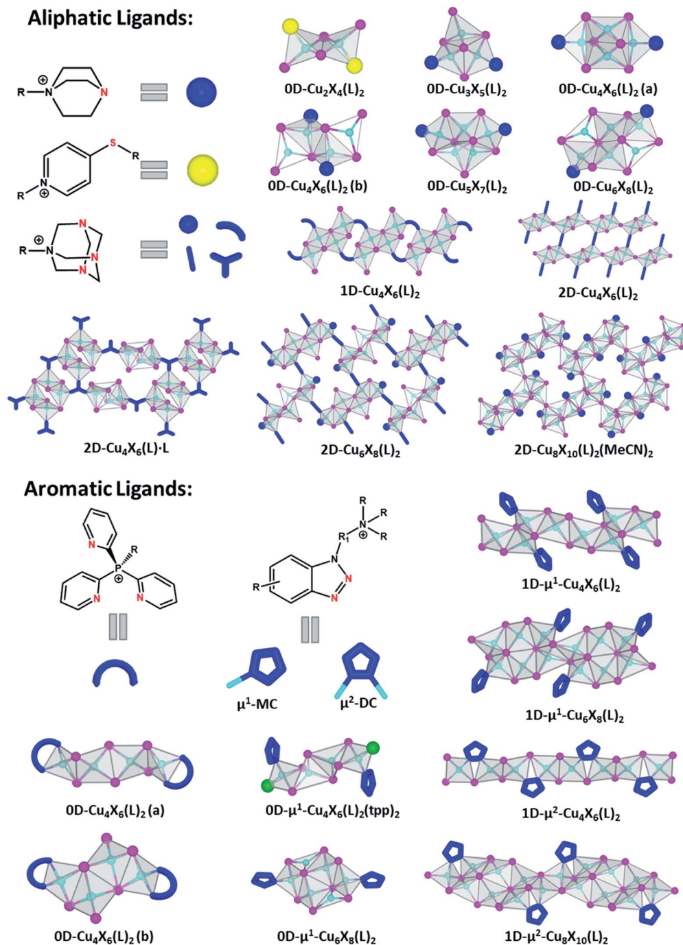
Fig. 1 Representative structures of AIO-type compounds. Color scheme: Cu, cyan; X, purple; P, green. Active coordination sites of the ligands (N and S) are marked in red.
