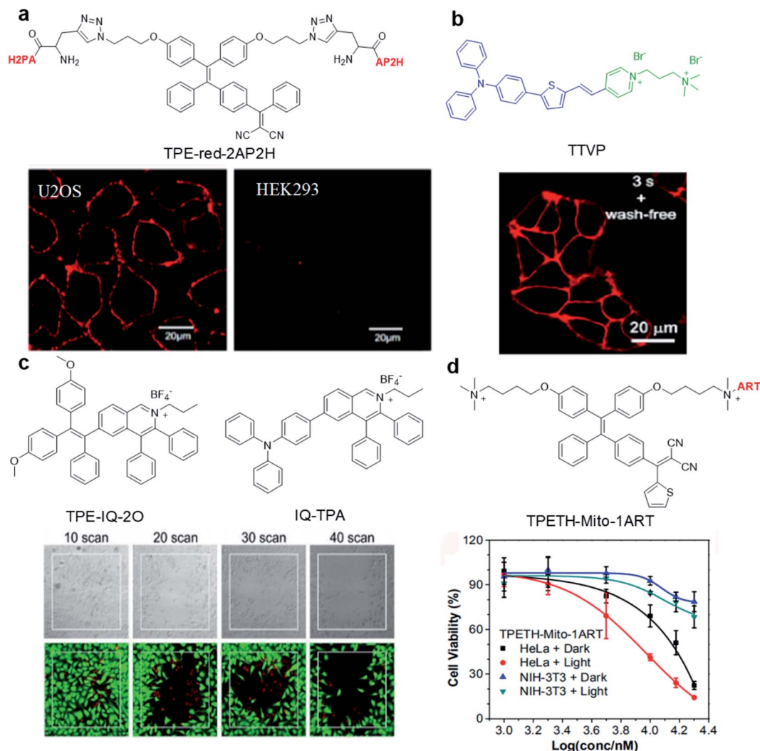
Fig. 3 (a) Chemical structure of TPE-red-2AP2H ; CLSM images of U2OS and HEK293 cells after incubation with TPE-red-2AP2H (10 \mu\text{M} ) in acidic environments. Reproduced from ref. 45 with permission. Copyright 2014 American Chemical Society. (b) Chemical structure of TTVP ; CLSM image of living HeLa cells after incubation with TTVP (500 nM). Reproduced from ref. 46 with permission. Copyright 2018 The Royal Society of Chemistry. (c) Chemical structures of TPE-IQ-2O and IQ-TPA ; live (green, FDA)/dead (red, PI) staining of IQ-TPA treated HeLa cells under two-photon scanning. Reproduced from ref. 51 with permission. Copyright 2018 The Royal Society of Chemistry. (d) Chemical structure of TPETH-Mito-1ART ; viabilities of HeLa and NIH-3T3 cells after treatment with TPETH-Mito-1ART for 2.5 h with or without white light treatment (60 \text{mW cm}^{-2} , 10 min). Reproduced from ref. 52 with permission. Copyright 2018 American Chemical Society.
