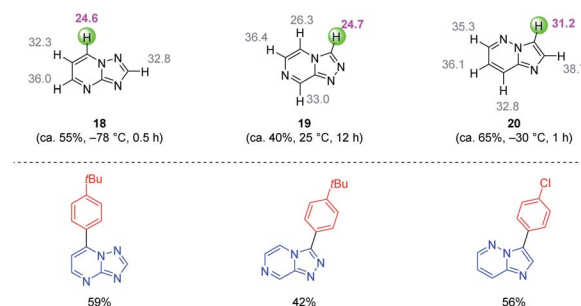
Scheme 6 Calculation of the \text{pK}_a -values of condensed N-heterocycles to predict their reactivity with \text{TMPZnCl} \cdot \text{LiCl} and subsequent quenching with electrophiles.
