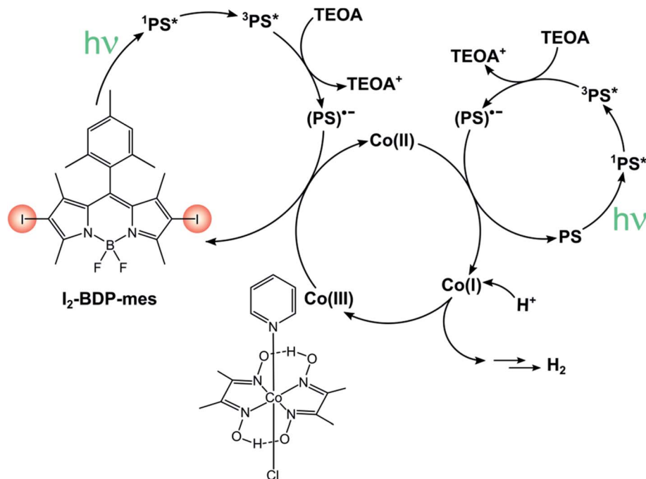
Scheme 18
