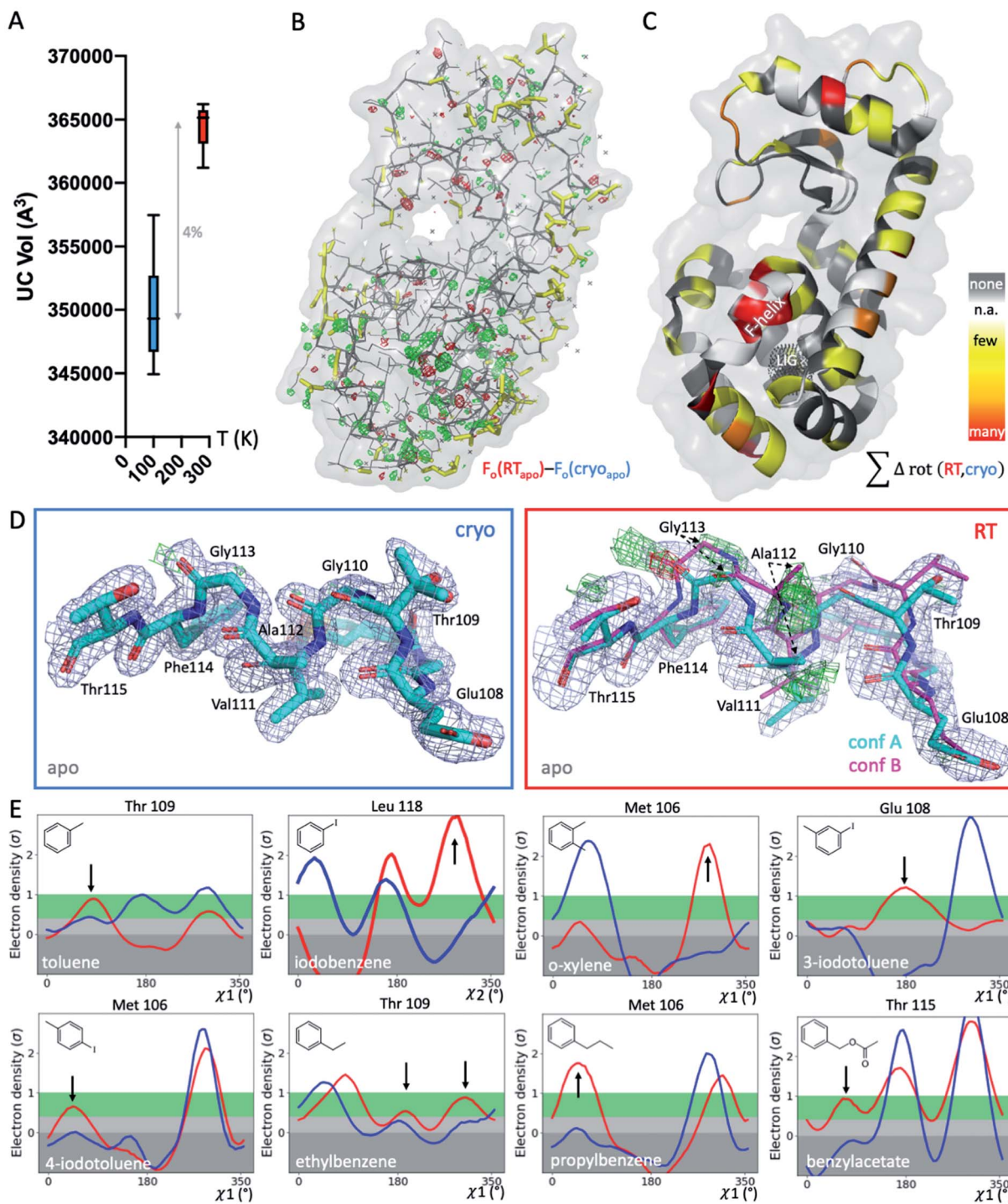
Fig. 1 Global and local structural responses to temperature. (A) Globally, structures at cryogenic temperatures (cryo; blue plot) are more variable and more compact than their room temperature (RT; red plot) equivalents, as shown by average unit cell (UC) volumes across 9 matched structures collected at both temperatures. (B) The isomorphous F_o - F_c map of the apo structure collected at cryo versus RT shows differences in the electron density (green mesh, positive difference electron density; red mesh, negative difference electron density) that indicate idiosyncratic temperature effects, especially around the ligand-binding site in the bottom lobe, indicated by the black dotted mesh in panel C (labeled LIG). (C) Occurrence of temperature-dependent rotamer differences across all 9 structures are projected onto the respective residues in the T4L apo structure; colored by temperature sensitivity of each residue across all 9 structure pairs: yellow for few structures, orange for several structures, and red for most structures showing temperature differences of the residue; white patches are Gly and Ala that do not have Chi angles; and grey patches show no rotamer change with temperature. (D) Locally, RT data of the L99A apo cavity reveal an alternative F-helix conformation (conf. B) in the F_o - F_c difference electron density maps (green and red mesh for positive and negative density, respectively; only cyan conformation A was included in refinement) that is not visible at cryo; 2mF_o - DF_c map shown as blue mesh; stick thickness represents relative occupancy. (E) All 8 ligand complexes show a shift in preferred orientation in response to temperature rather than due to ligand binding for at least 1 residue rotamer in the F-helix near the ligand-binding site. Ringer plots for selected residues, with rotamer differences at RT (red) versus cryo (blue) indicated by arrows.
