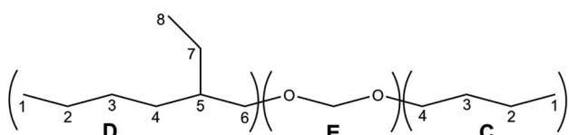
Scheme 2 Labelling for NMR analysis of (2-EH)BM.
