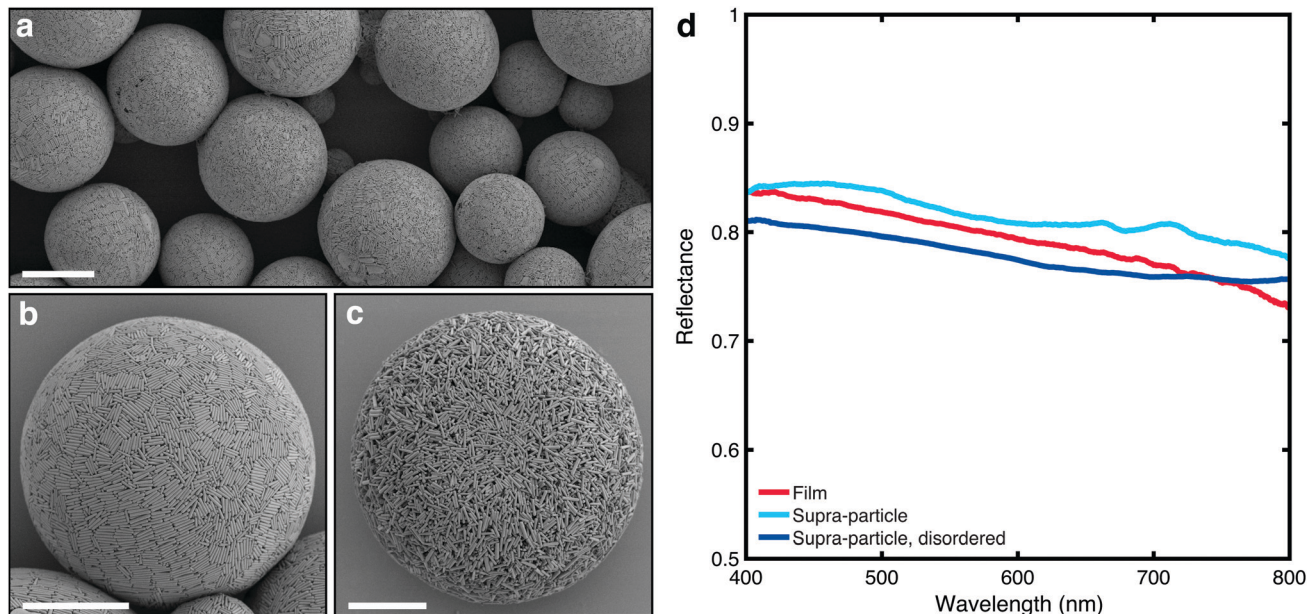
Fig. 2 SEM images and optical characterization of white silica supracolloidal balls. (a) low magnification SEM image of supracolloidal balls, (b) higher magnification image of single supracolloidal ball, (c) supracolloidal ball assembled in the presence of 10^{-2} M \text{CaCl}_2 . Scale bars: (a) = 15 \mu\text{m} (b and c) = 10 \mu\text{m} . (d) Reflectance spectra comparing the scattering properties of supraparticles with films of similar size (thickness of 25 \mu\text{m} ). Supraparticles show performance comparable to the corresponding films. Increasing the disorder reduces the scattering efficiency. The reflectance spectra for the supraparticles were measured using a microscope, while for the film they were retrieved from the total transmission data.
