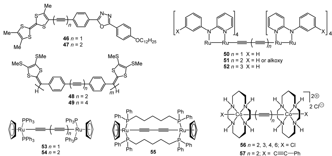
Fig. 16 Structures of 46–57 .
