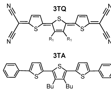
Scheme 4 Chemical structure of the quinoidal 3TQ in comparison with that of its aromatic counterpart, 3TA (Bu: n -butyl), a prototypical oligothiophene able to form \pi -dimeric dication.
