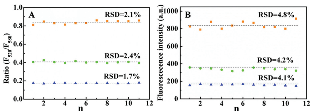
Fig. 3 11 parallel measurements of the CRISPR/Cas12a-based biosensing system in the presence of target DNA with different concentrations (0.025, 0.1, 0.25 nM from down to top) using the ratiometric probe (A) and TaqMan probe (B) as the reporter.
