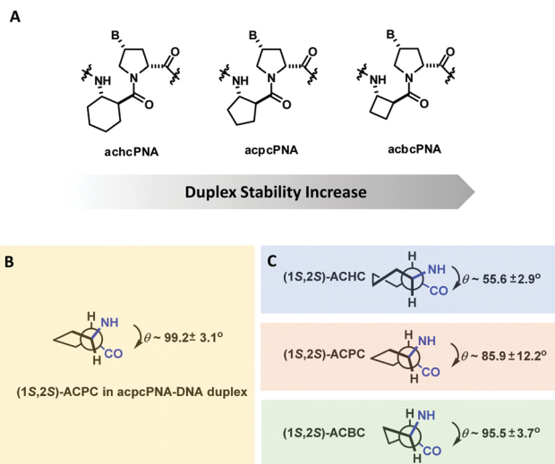
Fig. 27 (A) Structures of pyrrolidynyl PNA homologs. (B) Torsional angle N(H)–C \alpha –C \beta –C(O) of (1 S ,2 S )-ACPC in ACPC PNA. (C) Native torsional angles of cyclic \beta -amino acid oligomers are obtained from the literature (adapted with permission from ref. 137. Copyright 2012 American Chemical Society).
