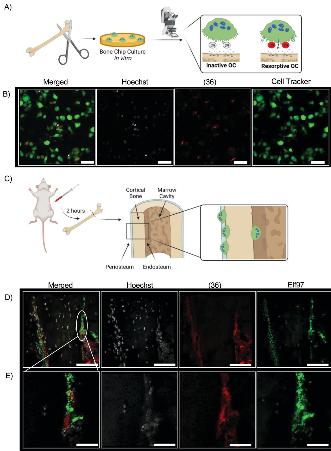
Fig. 6 Bisphosphonate targeting anchors (36) to the bone surface while maintaining the fluorescent properties of (3) when fluorescence is observed as a function of pH. To assess the abilities of (36) to detect osteoclast resorption in vitro , primary osteoclasts isolated from mice are cultured on bone chips and imaged by confocal laser microscopy, shown schematically (A). Osteoclasts are cultured on bovine bone chips with (36) for 24 hours and observed by confocal microscopy to determine local acidification (B, scale = 50 \mu m). In vivo , mice were injected with (36) by a tail vein injection and sacrificed two hours later; femurs were removed for non-decalcified histologic observation, shown schematically (C). In vivo bone resorption is observed by osteoclasts on the cortical bone surface of the femur (D, scale = 150 \mu m; E, scale = 30 \mu m) in mice injected with (36).
