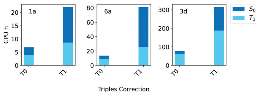
Fig. 5 Computation times in CPU hours for DLPNO-CCSD(T) calculations of the singlet ( S_0 , blue bars) and triplet state ( T_1 , light blue bars) of compounds 1a , 6a and 3d (Fig. 1) corresponding to T0 and T1 triples corrections. In all cases, the aug-cc-pVTZ basis set and TightPNO settings were used.
