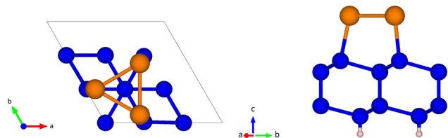
Fig. 1 (Left panel) Top and (right panel) side views of the slab model of the Si(111)-( \sqrt{3} \times \sqrt{3} )R30°-Sb surface with the bottom layer saturated by hydrogen atoms. In the top view the surface unit cell is shown with Si atoms in the first, second and fourth layers. The three Sb atoms in the surface unit cell (orange spheres) form a trimer with its centroid aligned with the Si atom in the fourth layer. Si, Sb and H atoms are shown by blue, orange and pink spheres, respectively.
