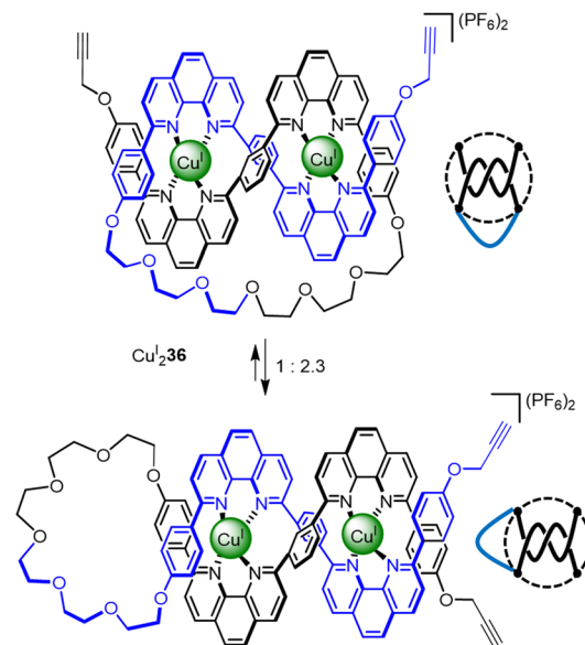
Fig. 12 Molecular overhand knot \text{Cu}_2 36 and its tangle representation. The complex was generated along with a sequence isomer. The undesired denominator closure in the sequence isomer means that the synthon only generates nugatory crossings which untwist upon demetallation. 72
