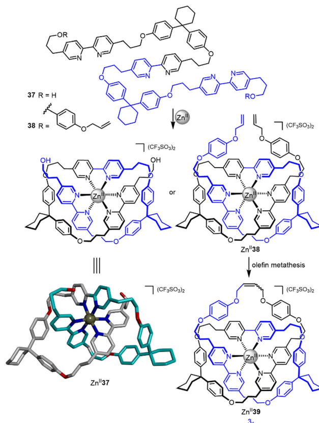
Fig. 13 Synthesis of overhand knot \text{Zn}_3^{\text{II}} 37 and trefoil knot \text{Zn}_3^{\text{II}} 39 by folding of a single ligand strand around a \text{Zn}^{\text{II}} ion. 75,76
