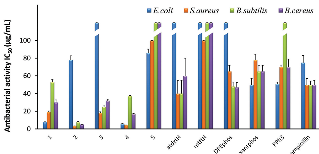
Fig. 3 In vitro antibacterial activity of 1–5 , and their ligands atdztH, mtfH, DPEphos, xantphos, and PPh 3 in free form, expressed as half-minimum inhibitory concentration (IC 50 ) values ( \mu\text{g mL}^{-1} ) provided by a nonlinear curve fit-growth/sigmoidal-dose response on the experimental optical density data. Values are expressed as mean \pm standard deviation (SD) of three replicate measurements (with the exception of values higher than 100 \mu\text{g mL}^{-1} ).
