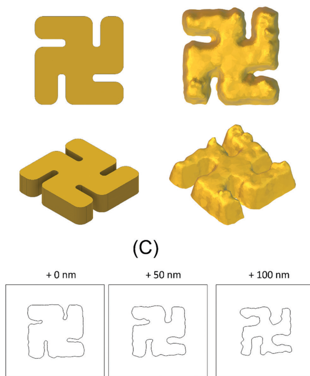
Fig. 2 A plan and 3-D view of the (A) ideal and (B) real models of LH gammadion nanostructures used in numerical simulations. (C) Cut slice profile of the 'real' structure 0, 50 and 100 nm above the glass substrate. The structure shows significant sloping.
