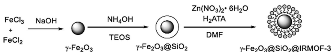
Fig. 29 Schematic showing the preparation of the \gamma-Fe_2O_3@SiO_2/IRMOF-3 catalyst. This figure was adapted with a permission from Journal of Catalysis , 2020, 387, 39–46. 188
