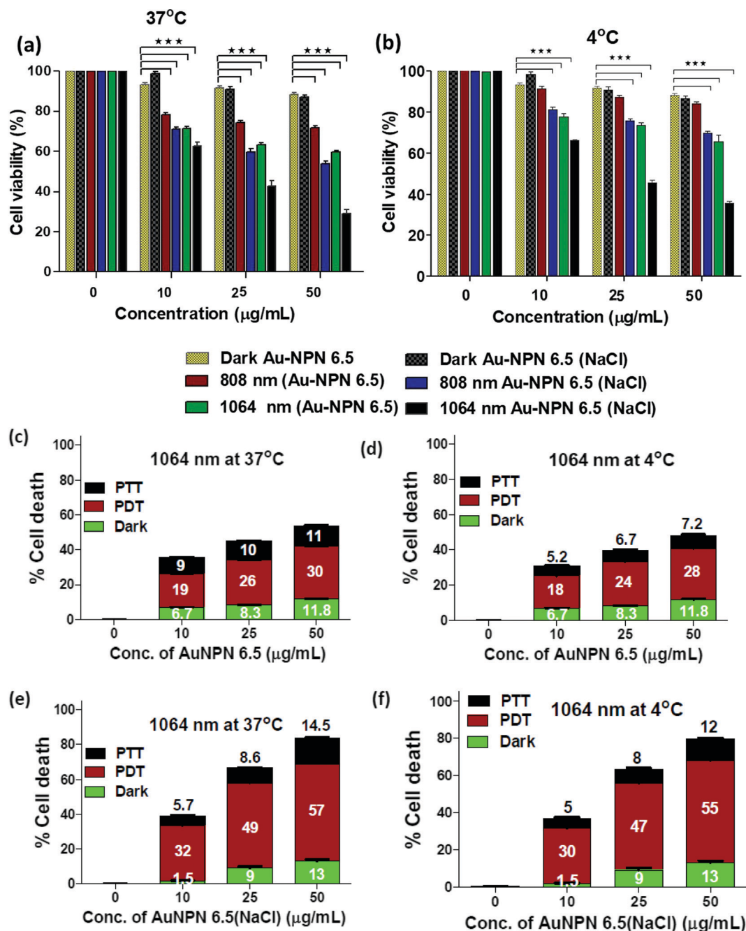
Fig. 4 Cell viability of Au NPN6.5 upon 1064 nm NIR light irradiation at 37 °C and 4 °C. Cell viability assay for Au NPNs at different conditions in murine CT-26 colon carcinoma cancer cells: (a) Au-NPN6.5 and Au NPN6.5(NaCl) at 37 °C and (b) Au-NPN6.5 and Au-NPN6.5(NaCl) at 4 °C. Relative contributions of PDT and PTT to cellular death under 1064 nm photo irradiation of (c) Au-NPN6.5 at 37 °C, (d) Au NPN6.5 at 4 °C, (e) Au NPN6.5(NaCl) at 37 °C, and (f) Au NPN6.5(NaCl) at 4 °C.
