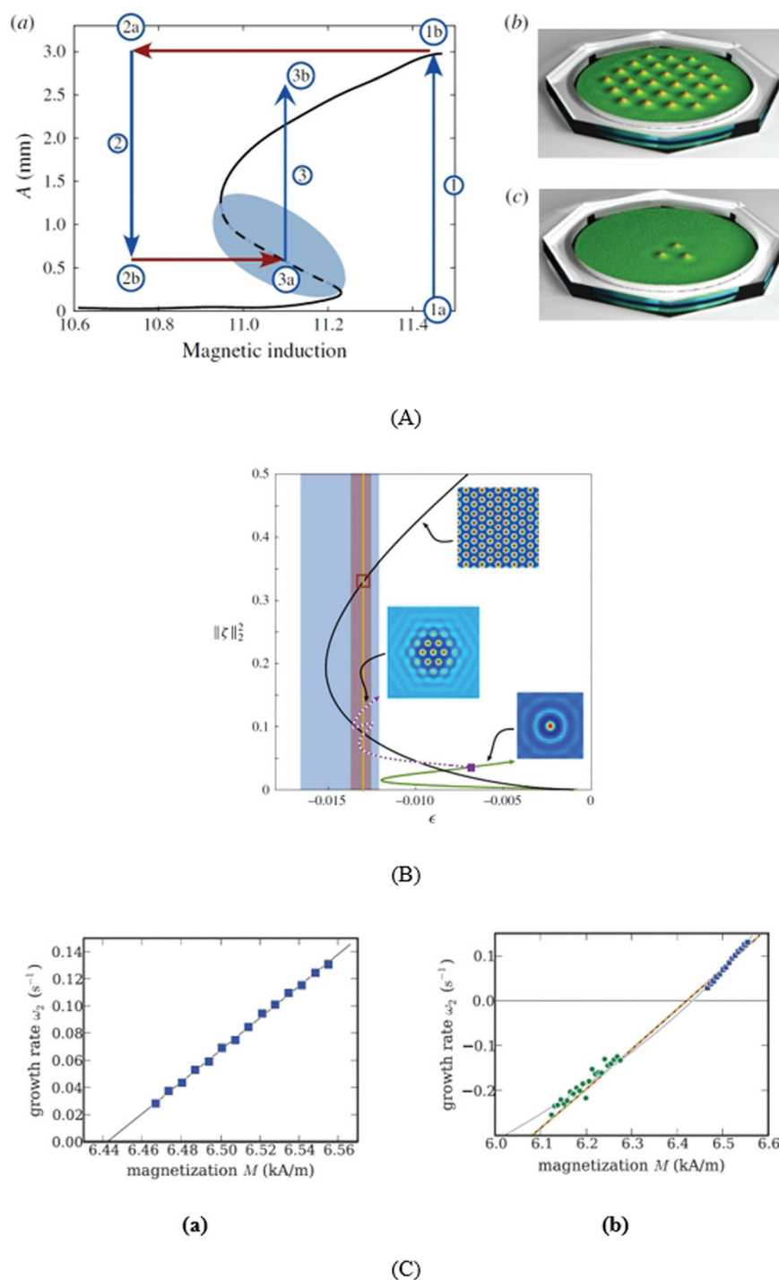
Fig. 31 Rosensweig instability patterns in a highly viscous ferrofluid. (A) (a) The bifurcation diagram (black line) of this pattern is obtained by a fitting procedure of amplitude equations described in ref. 555 to about 170 000 measured data. Via the path indicated by the arrows, one obtains localized patches, as shown in (c). The magnetic induction B is kept fixed during (1) for a time delay of \tau_1 , and then B is switched to (2) for a time delay of \tau_2 before finally being switched to (3) until equilibrium is reached at point (3b). (b) A reconstruction of the height field of the domain-covering hexagons at point (1b). (c) Gives a reconstruction of the height field of a three-spike patch at point (3b) in the bifurcation diagram. (B) Emergence of a fully localized hexagon patch (dashed purple) bifurcating from a single spike (green) with \mu_r = 2 . There are also plotted the snaking regions of the \langle 10 \rangle (blue) and \langle 11 \rangle planar fronts (red); here, \epsilon denotes the bifurcation parameter, which depends on the relative permeability of the ferrofluid, \mu_r (reproduced from ref. 556 with permission from Cambridge Univ. Press, copyright 2015). (C) Grow and decay of the Rosensweig pattern in the case of a highly viscous ferrofluid. (a) The linear growth rates \omega_2 (■) from the experiment and the maximal growth rate \omega_{2,m} (solid black line) from theory as a function of the magnetization M . (b) The growth (■) and decay (●) rates \omega_2 of the pattern amplitude as a function of the magnetization M . The symbols represent the measured data. The black dashed line shows a fit of expression of scaling law for \omega_2 to the experimental growth and decay rates (reproduced from ref. 554 with permission from Am. Phys. Soc., copyright 2016).
