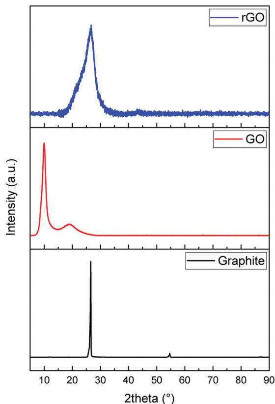
Fig. 1 XRD patterns of graphite, GO and rGO.
