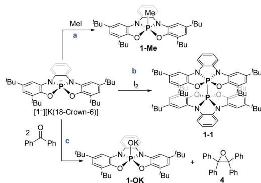
Scheme 3 Preliminary reactivity study of phosphorane 1^- .
