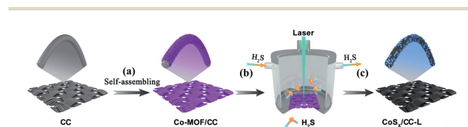
Scheme 1 Schematic illustration of the fabrication process of \text{CoS}_x/\text{CC-L} using a laser combined with a \text{H}_2\text{S} atmosphere (b and c) from Co-MOF/CC (a).
