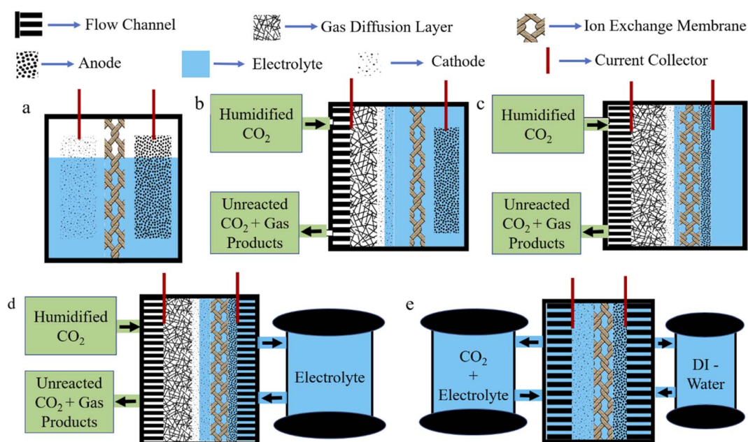
Fig. 4 Graphical representations of (a) a conventional H-type cell, (b) a GDE cell, (c) an MEA cell, (d) a zero-gap MEA cell, and (e) an MEA flow cell.
