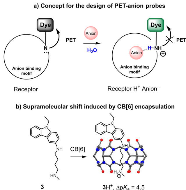
Fig. 2 (a) Design concept of a fluorescent receptor for anions with a “turn-on” response. (b) Example of the supramolecular complexation of the pH probe in the cavity of cucurbit[6]uril.
