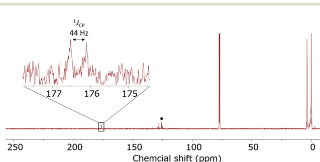
Fig. 8 ^{13}\text{C}\{^1\text{H}\} NMR spectra for the reaction of (\text{Me}_3\text{Si})_3\text{P}_7 with \text{CO}_2 . Dissolved \text{CO}_2 marked with *.
