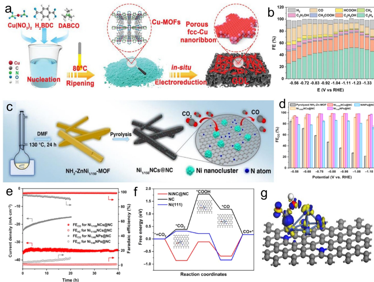
Fig. 20 (a) Synthesis scheme of Cu-MOFs and porous Cu nanoribbons. (b) FEs for Cu nanoribbons. Reproduced with permission from ref. 195 Copyright 2021, Wiley. (c) Synthesis of Ni 1/150 NCs@NC catalyst. (d) FEs. (e) Stability tests. DFT calculation for CO 2 electrocatalytic reduction: (f) free-energy diagram for different models. (g) Depiction of electron density difference between Ni cluster and *COOH intermediate. Reproduced with permission from ref. 68 Copyright 2022, Springer.
