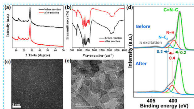
Fig. 30 (a) XRD and (b) FT-IR patterns of CoNiS x -CN before and after the photocatalytic H 2 evolution reaction. 118 (c) The spherical aberration-corrected HAADF-STEM image of Ce-SA-C 3 N 4 after the photocatalytic hydrogen evolution from water splitting cycle experiments. 99 (d) N 1s core-level XPS spectra of W-PCN600 before and after the cyclic OWS experiment. 128 (e) TEM image of PtSA-CN620 after the photocatalytic H 2 production reaction. 129
