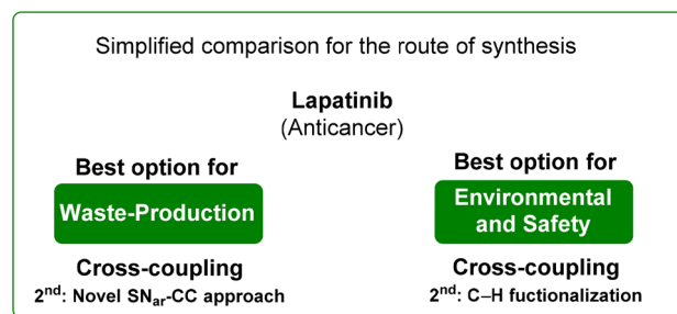
Scheme 40 Summarised assessment for lapatinib synthesis.
