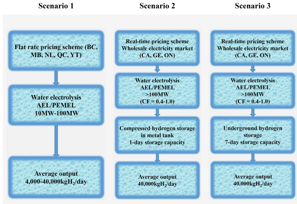
Fig. 20 Deployment scenarios for water electrolysis. (BC = British Columbia; MB = Manitoba; NL = Newfoundland and Labrador; ON = Ontario; QC = Quebec; YT = Yukon; CA = California; GE = Germany.) Modified from ref. 233 with permission from Elsevier, copyright 2019.
