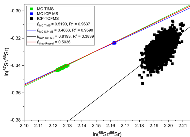
Fig. 4 Three-isotope plot for Sr from measurements over several hours of NIST SRM 987 using ICP-TOFMS (integration time 0.5 s, M = 2000 ), MC TIMS (integration time 24 s, M = 443 ) and MC ICP-MS (integration time 42 s, M = 238 ). Solid lines represent experimentally determined slopes ( \beta_{\text{instrument}} ) and predicted mass dependent fractionation line ( \beta_{\text{theo-Russell}} ). All data points were taken from measurements of pure NIST SRM987 single-element solution.
