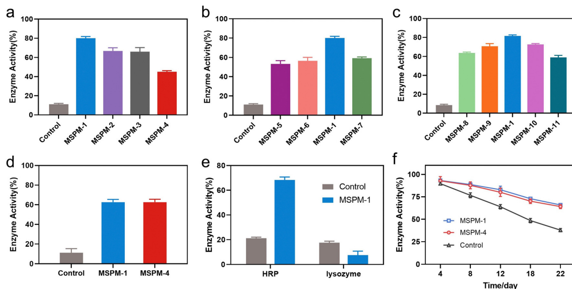
Fig. 3 Nanochaperones protect proteins from thermal denaturation. (a), (b) and (c) The recovered enzyme activity of thermally denatured HRP (50 \mu\text{g mL}^{-1} ) in the absence (control) or presence of MSPMs (0.5 \text{mg mL}^{-1} ) after being heated at pH 7.4, 85 °C for 1 h. (d) The recovered enzyme activity of thermally denatured lysozyme (50 \mu\text{g mL}^{-1} ) in the absence (control) or presence of self-co-nChap (MSPM-1) or non-specific nChap (MSPM-4) (0.5 \text{mg mL}^{-1} ) after being heated at pH 7.4, 85 °C for 1 h. (e) The recovered enzyme activity of HRP and lysozyme in the absence (control) or presence of self-co-nChap (MSPM-1) (0.5 \text{mg mL}^{-1} ) after the HRP (50 \mu\text{g mL}^{-1} ) and lysozyme (50 \mu\text{g mL}^{-1} ) mixture was heated at pH 7.4, 80 °C for 1 h. (f) The residual enzyme activity of HRP (50 \mu\text{g mL}^{-1} ) in the absence (control) or presence of self-co-nChap (MSPM-1) or non-specific nChap (MSPM-4) (0.5 \text{mg mL}^{-1} ) after being heated at pH 7.4, 40 °C for different times.
