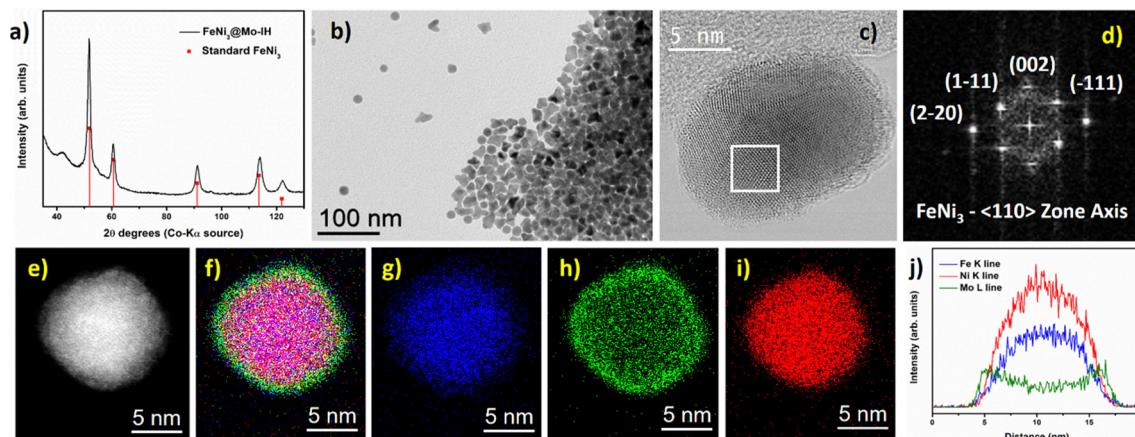
Fig. 4 \text{FeNi}_3 @Mo-IH NPs: (a) powder XRD pattern (ICDD: 00-038-0419, red vertical drop lines for standard \text{FeNi}_3 ), (b) BF TEM micrograph, (c) HRTEM image of a single nanoparticle, (d) FFT pattern of the marked white square zone from HRTEM figure c along \langle 110 \rangle zone axis, (e) STEM-HAADF image, (f)–(i) individual STEM-EDX maps showing Fe in blue, Ni in red, and Mo in green, and their overlap map, and (j) line scan profile of a single nanoparticle obtained using STEM-EDX technique (Mo L line – green, Fe K line – blue, and Ni K line – red).
